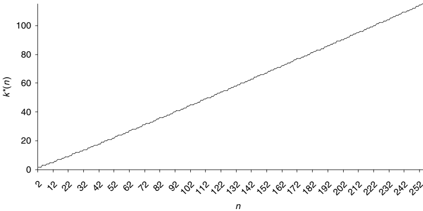
Fig. 1. Relationship between the number of dimensions ( n ) and the maximum amount of dimensions that must be won for the existence of equilibrium ( k^*(n) )
